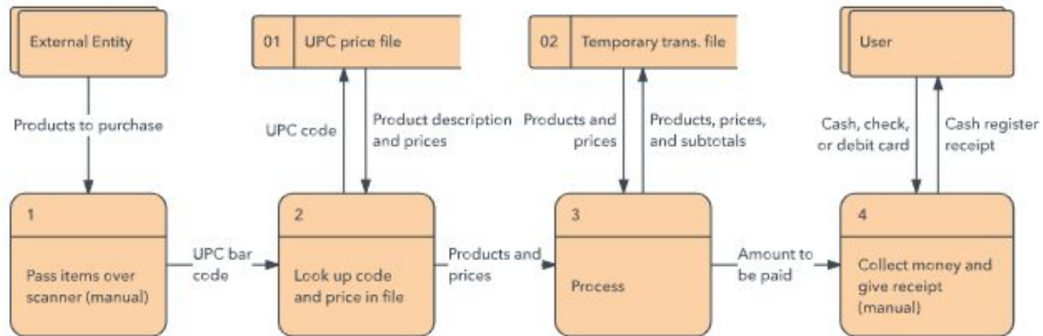
Physical DFD
